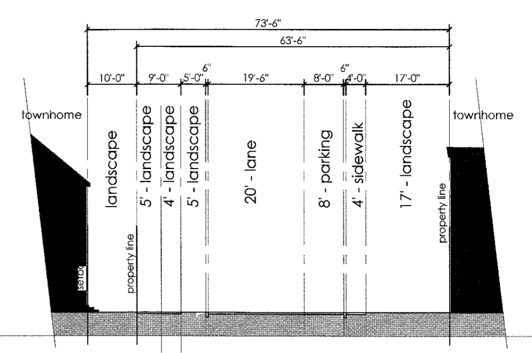
5 Street Cross Section 1" = 20'-0"
