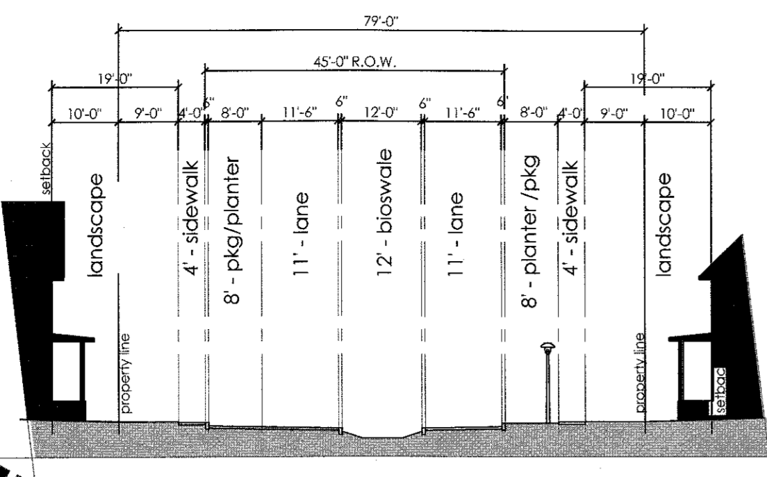
1 Boulevard Cross Section 1" = 20'-0"
