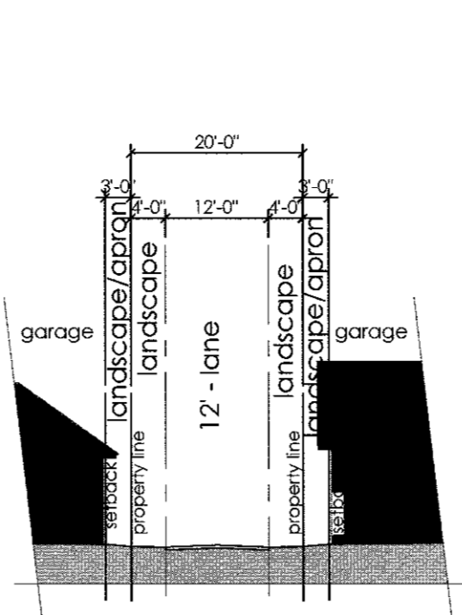
3 Alley Cross Section 1" = 20'-0"
