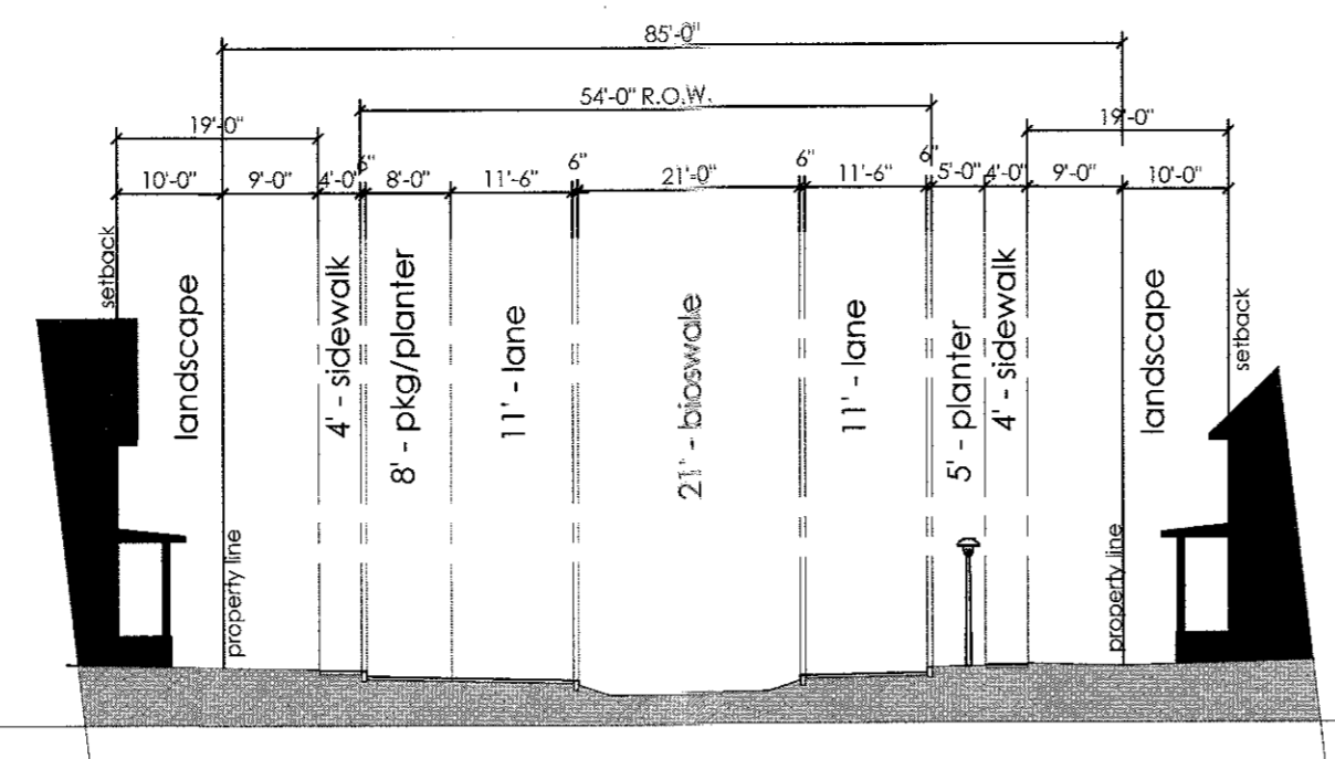
2 Boulevard Cross Section 1" = 20'-0"
