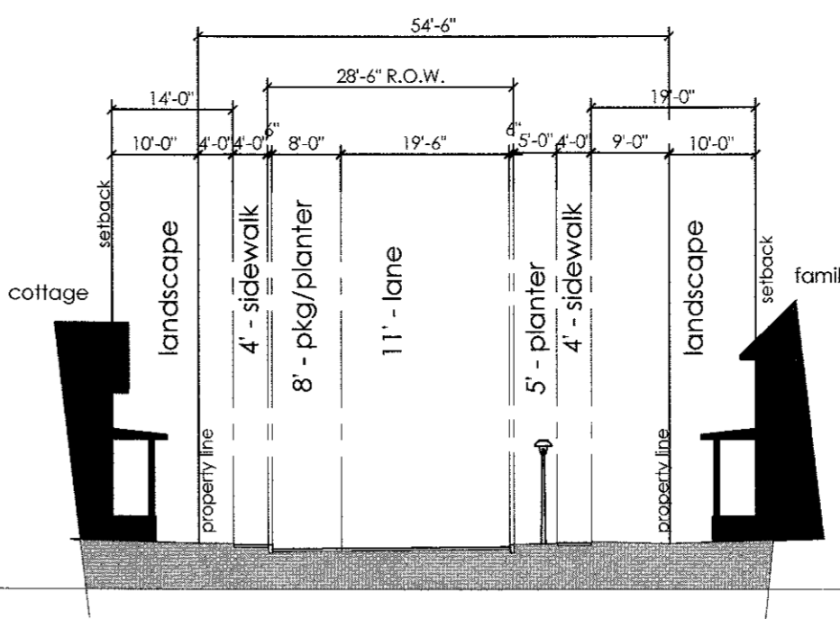
4 Street Cross Section 1" = 20'-0"
